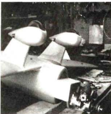
Fiberglass parts for the STA can either be formed as described in text or obtained from Fiberglass Master.
